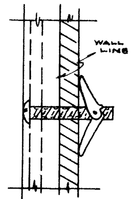
TOGGLE BOLTS FOR HOLLOW TILE MOUNTING OR METAL LATHE AND PLASTER
